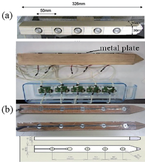
図 2. 縦挿し型送受信機 (a) transmitter, (b) receiver.
