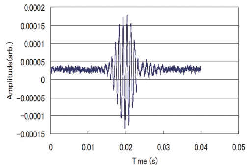
図 4. Received wave form: 18 cm distance, 10 cm depth, 1000 Hz and 5 cycles.
