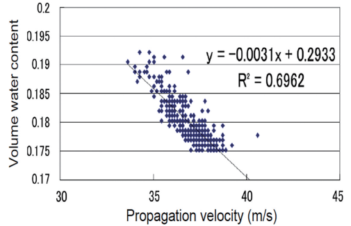
図 7. Relation between propagation velocity and volume water content.
