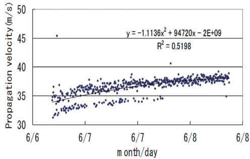
図 6. Propagation velocity change.
