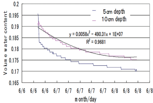
図 5. Volume water content change.
